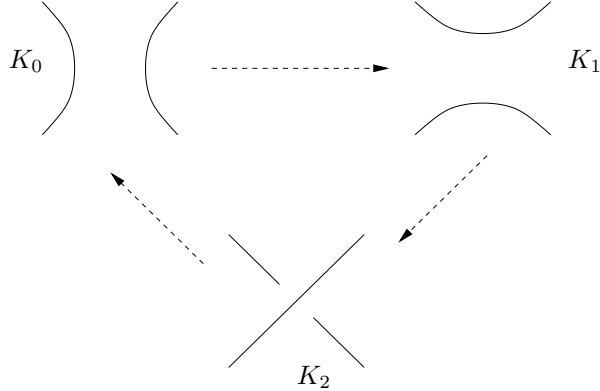
FIGURE 1. The links K_0 , K_1 , K_2 comprise an unoriented skein triple.
