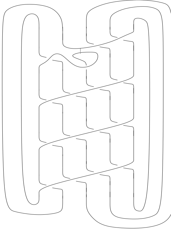
FIGURE 2. The dotted line represents a blackboard-framed 1-handle attachment which gives a knot cobordism from the knot 5_2 to T(4, 5) .
