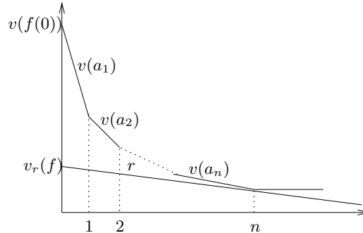
FIGURE 2. An illustration of the “ p -adic Jensen formula”. The numbers over each line are their slopes.
