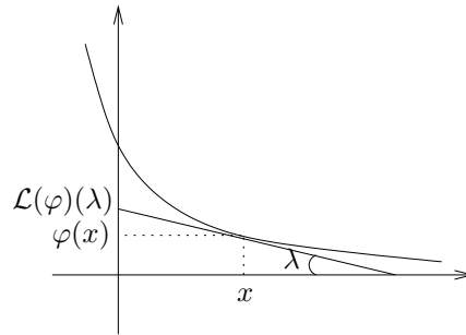
FIGURE 1. The Legendre transform of \varphi evaluated at the slope \lambda where by definition the slope is the opposite of the derivative (we want the slopes to be the valuations of the roots for Newton polygons).
