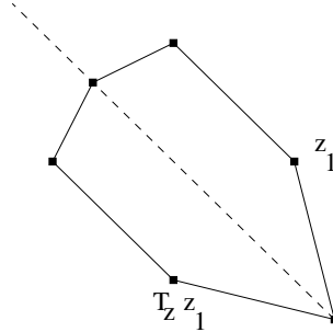
FIGURE 2. Three links being reflected in the dotted line.
