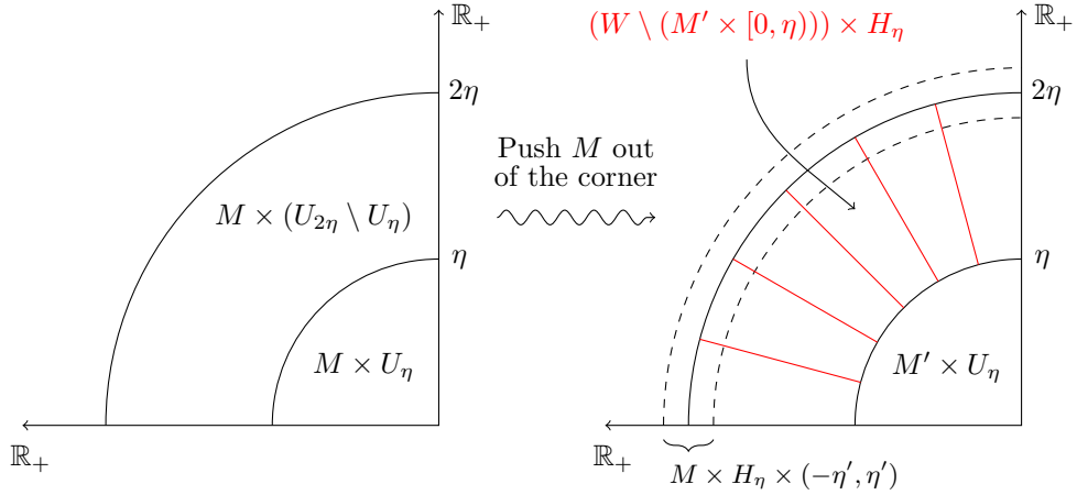
FIGURE 2. Example of pushing M out of the corner. Here N = 2 and \mathbb{E}^d is thought of as the direction perpendicular to the page. Each radial red line is a copy of W (minus a collar at the M' boundary). Note the outer “shell” M \times H_\eta \times (-\eta', \eta') , after the push, could also be considered to be a copy of M \times H_{2\eta} \times (-\eta', \eta') due to the radial dilation in the embedding \iota_Y .
