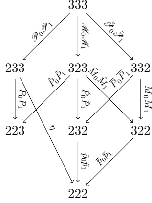
FIGURE 6. The framed flow category \mathcal{C}_2 .
