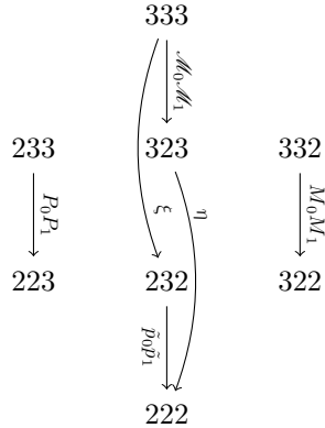
FIGURE 9. The flow category \mathcal{C}_5 . The middle summand corresponds to a special cyclic word in the sense of Baues–Hennes [BH91].
