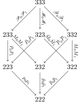
FIGURE 5. A subcategory \mathcal{C}_1 of \mathcal{L}^{\text{Kh}}(L) .
