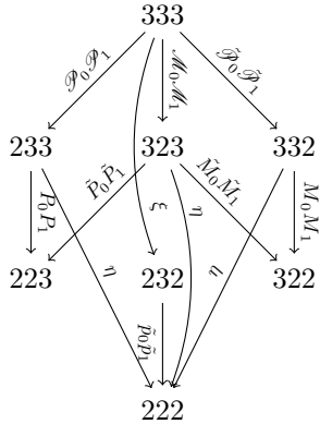
FIGURE 7. The framed flow category \mathcal{C}_3 .
