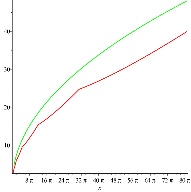
Figure 1: The graphs of the function from Proposition 3.3 (green) and the functions from [2] (red) in the case of \alpha = (\sqrt{5} + 1)/2 = [1; 1, 1, 1, \dots] . In this case we take q_N = 2 , \lambda_N = q_N/q_{N+1} = 2/3 and t = 1 . (Compare Figure 2 of [2].)
