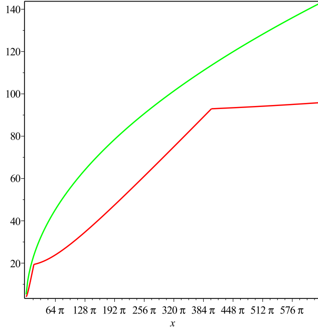
Figure 2: The graphs of the function from Proposition 3.3 (green) and the functions from [2] (red) in the case of \alpha = (\sqrt{21} + 3)/6 = [1; 3, 1, 3, \dots] . In this case we take q_N = 4 , \lambda_N = (\sqrt{21} - 3)/2 and t = 1 . (Compare Figure 3 of [2].)
