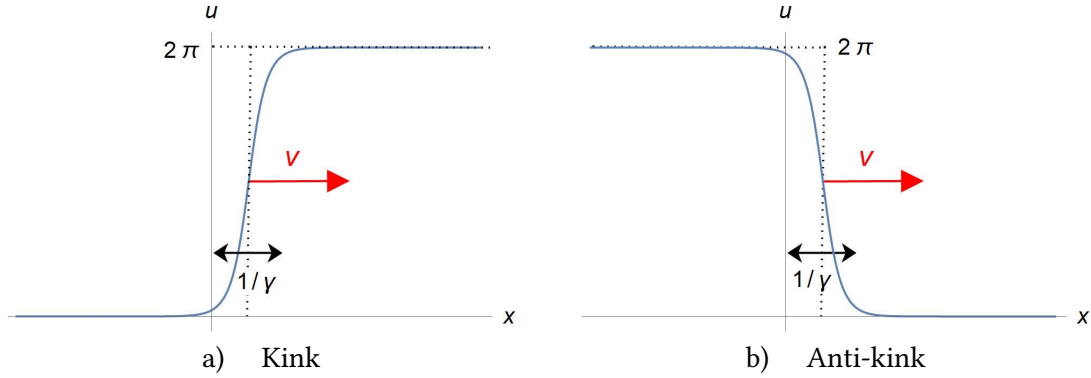
Figure 3.2: Snapshots of the sine-Gordon kink and anti-kink.
