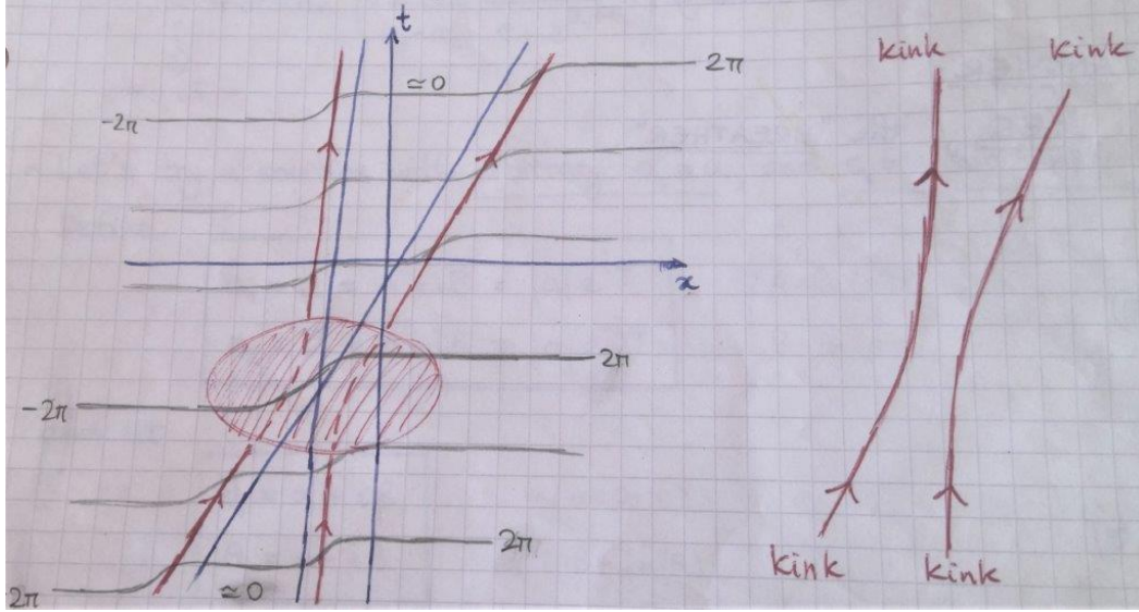
Figure 6.4: Schematic summary of the kink-kink solution.
