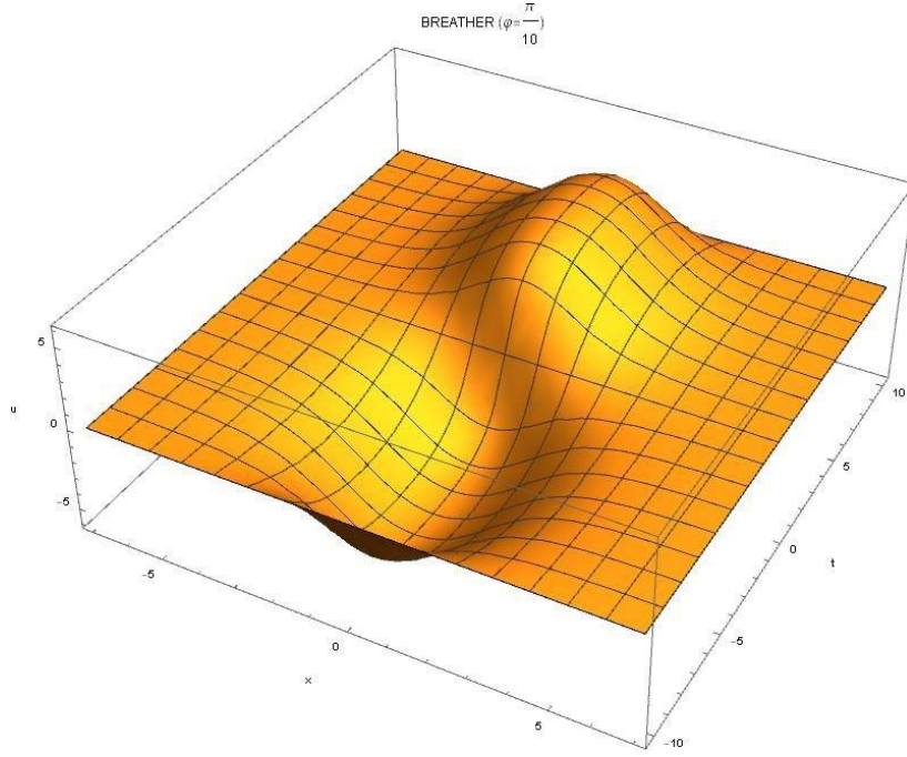
Figure 6.8: 3d plot of the breather solution for v = 0 and \varphi = \pi/10 .
