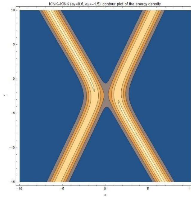
Figure 6.6: Contour plot of the energy density of the a_1 = 0.6 , a_2 = -1.5 solution.
