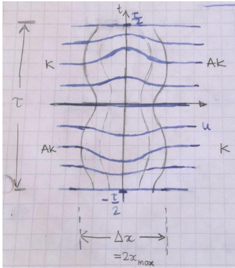
Figure 6.7: Sketch of the v = 0 breather solution.
