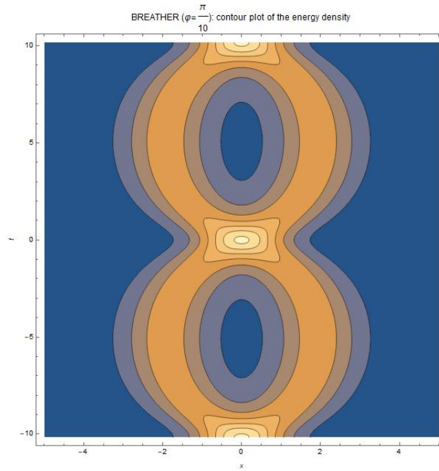
Figure 6.9: Contour plot of the energy density of the v = 0 , \varphi = \pi/10 breather.
