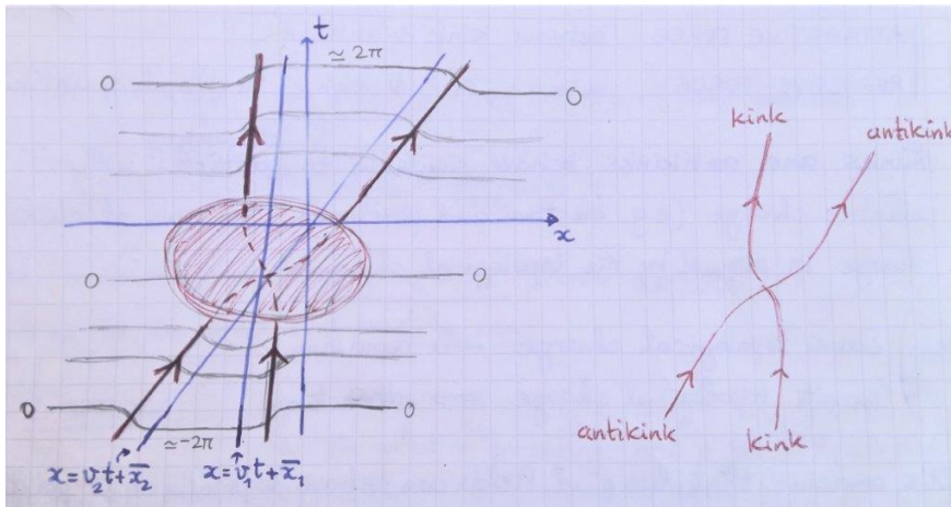
Figure 6.1: Schematic summary of the kink-antikink solution.
