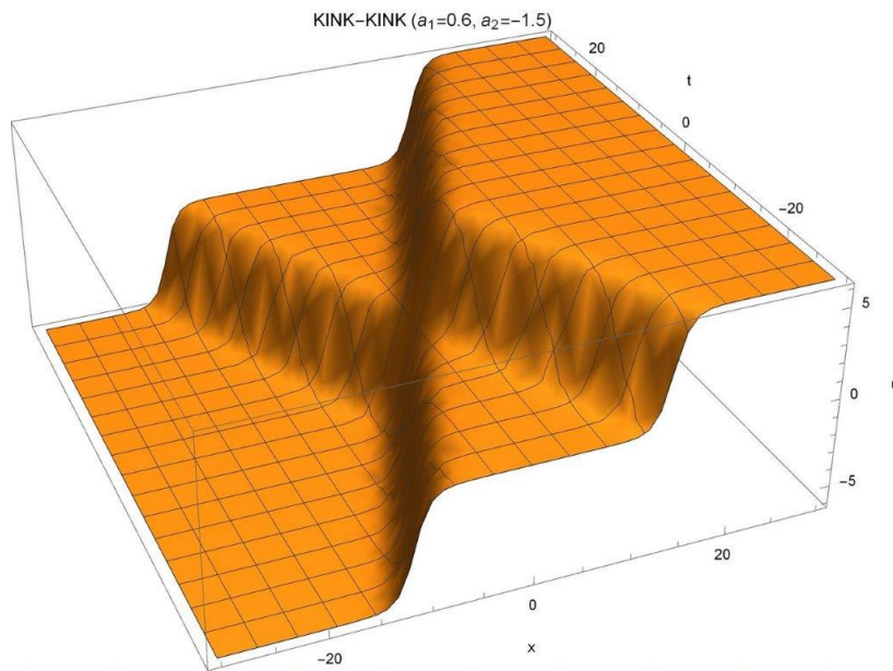
Figure 6.5: 3d plot of the kink-kink solution for a_1 = 0.6 , a_2 = -1.5 .
