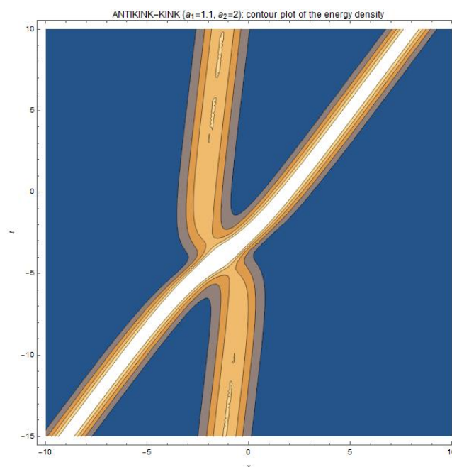
Figure 6.3: Contour plot of the energy density of the a_1 = 1.1 , a_2 = 2 solution.
