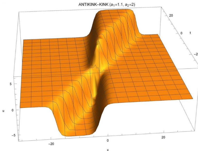
Figure 6.2: 3d plot of the kink-antikink solution for a_1 = 1.1 , a_2 = 2 .
