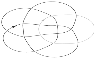
FIGURE 1. The link L_3 .
