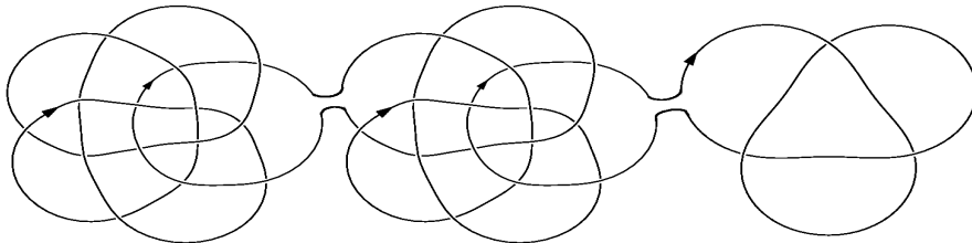
FIGURE 2. The link L_3^2 .
