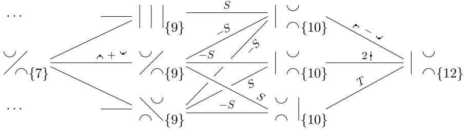
FIGURE 6. The cochain complex E^* .
