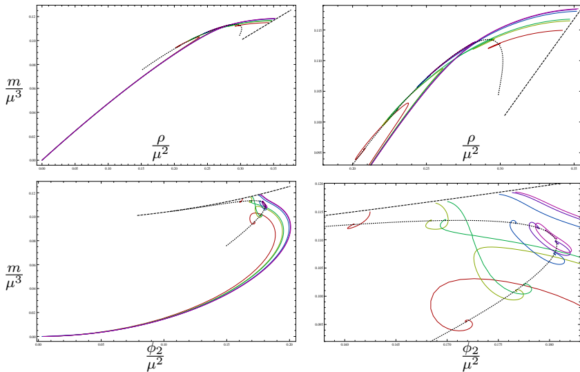
Figure: Scale-invariant quantities. The right panels zoom in to the interesting bits.
