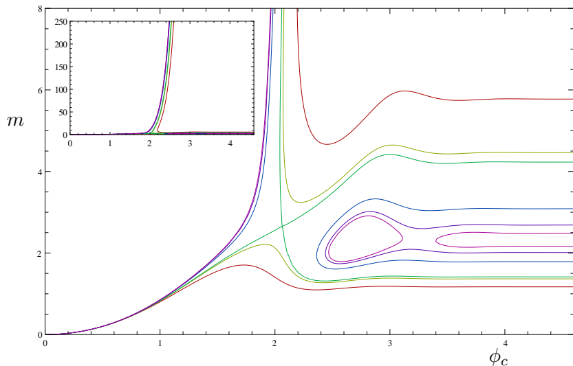
Figure: Contours of the function q(m, \phi_c) — colour represents the value of q . Inset is the behaviour over a large range of m .
