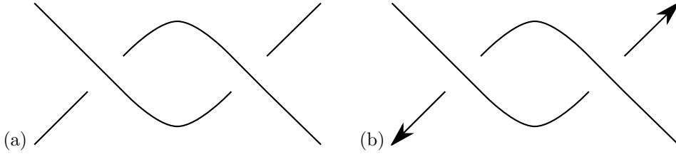
FIGURE 5. The basic matched tangle, (a) unoriented and (b) oriented.
